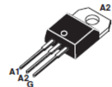
TO-220B(BTB06)
