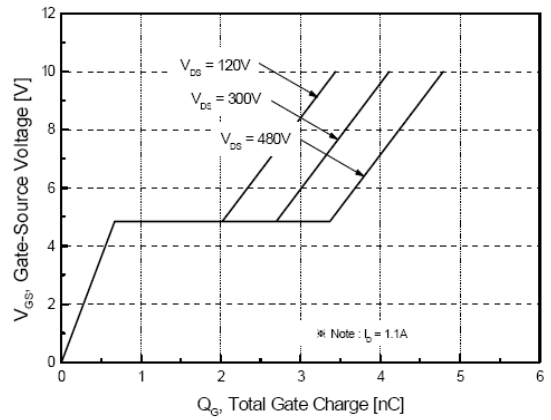
图6. 栅电荷特性曲线 Fig. 6 Gate Charge Characteristics
